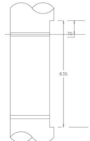
DETAIL B SIDE ELEVATION NTS
